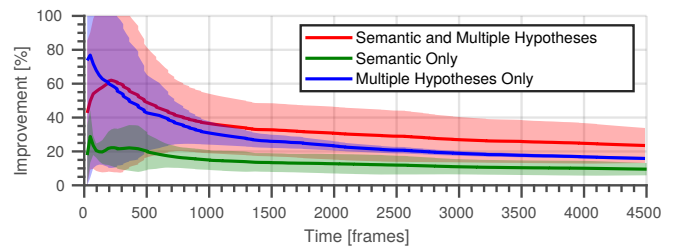
Fig. 8: Reduction of the RMSE for a single hypothesis, non-semantic DPMHM. Including both modalities, we achieve an average reduction of 34 %, with only multiple hypotheses 27 % and 13 % with a pure semantic DPMHM.
