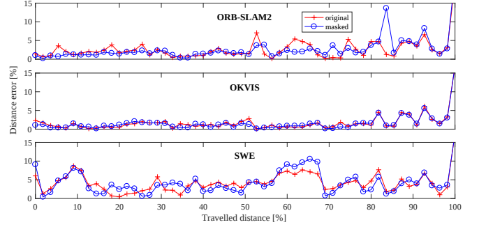
Fig. 8. Distance errors using the whole image (red) and masked out visual aliasing areas (blue).
