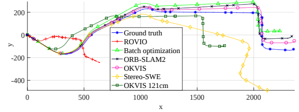
Fig. 6. Path alignment of trajectory estimations of the different motion estimation pipelines on trajectory2 . If not stated otherwise, the 31 cm baseline is displayed. Due to the unrecoverable resets of the estimator, VINS-Mono is omitted here.
