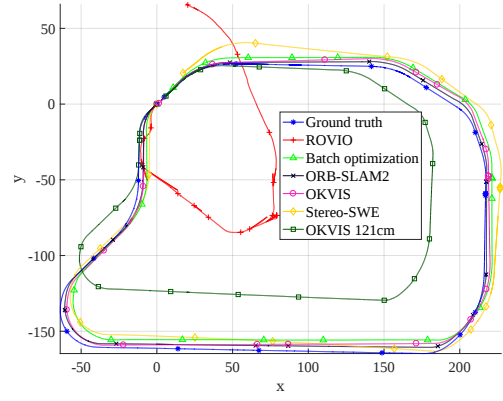
Fig. 5. Path alignment of trajectory estimations of the different motion estimation pipelines on trajectory1 . If not stated otherwise, the 31 cm baseline is displayed. Due to the unrecoverable resets of the estimator, VINS-Mono is omitted here.
