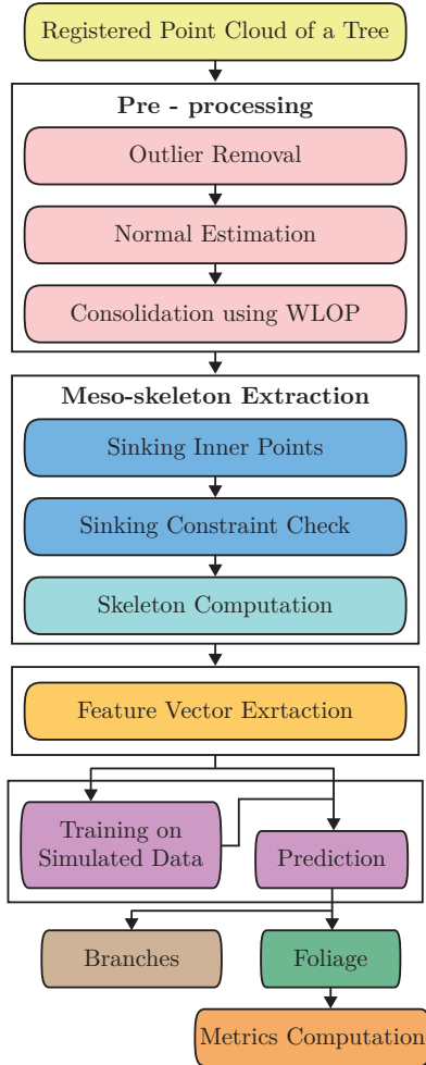
Fig. 2: An overview of the proposed algorithm.
