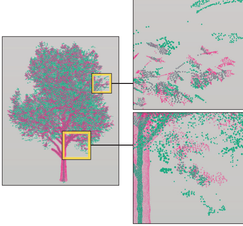
(a) Figure shows the inner points (in green) computed by the unmodified Deep Points algorithm. The inner points move far away from the surface points (in red) for leaves.
